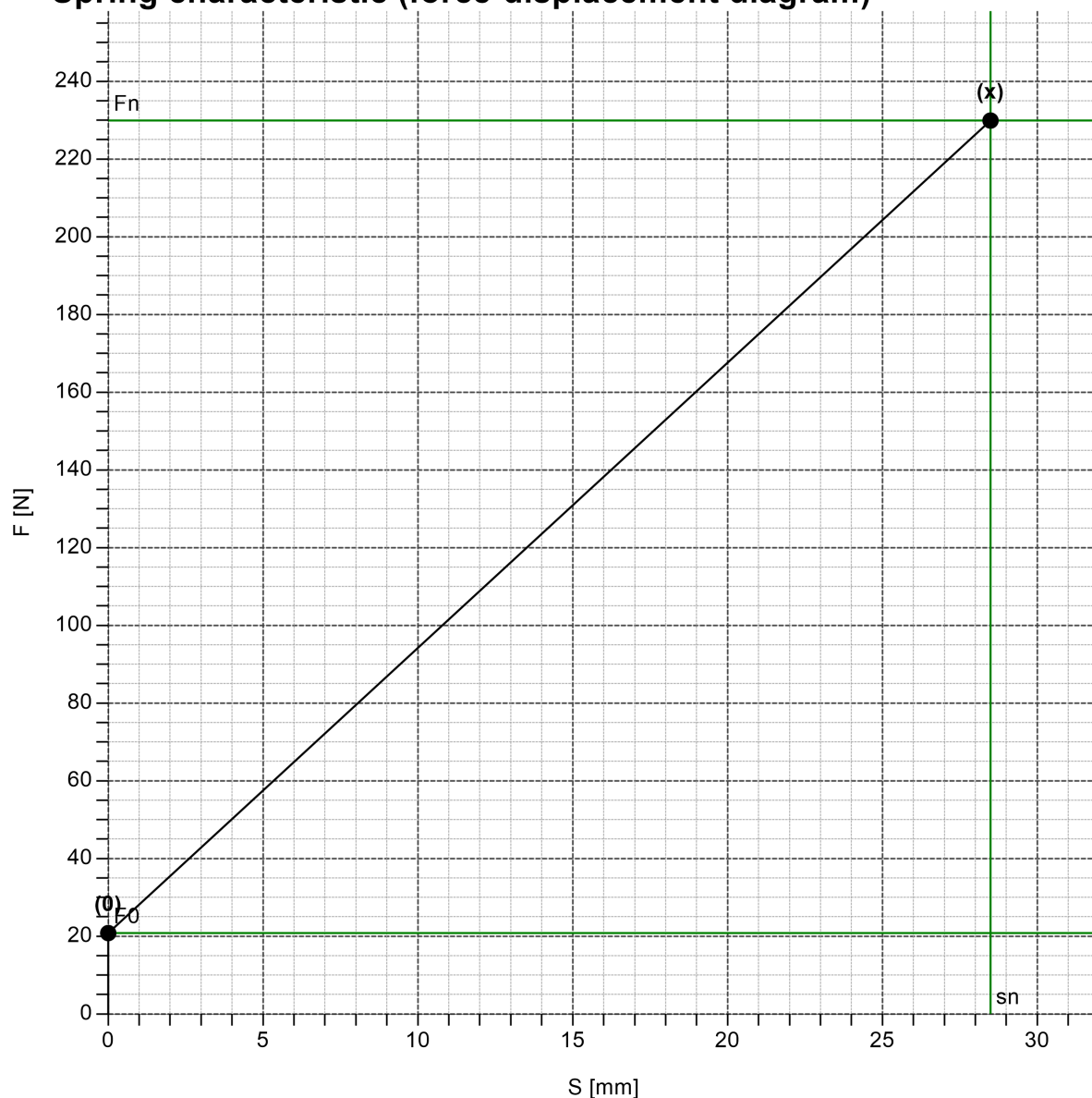
Spring characteristic (force-displacement diagram)
