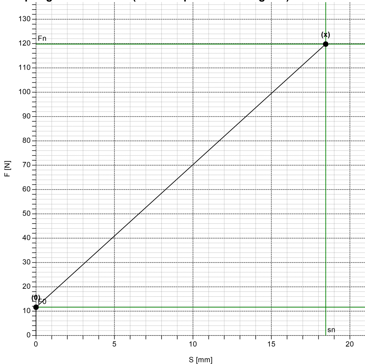
Spring characteristic (force-displacement diagram)
